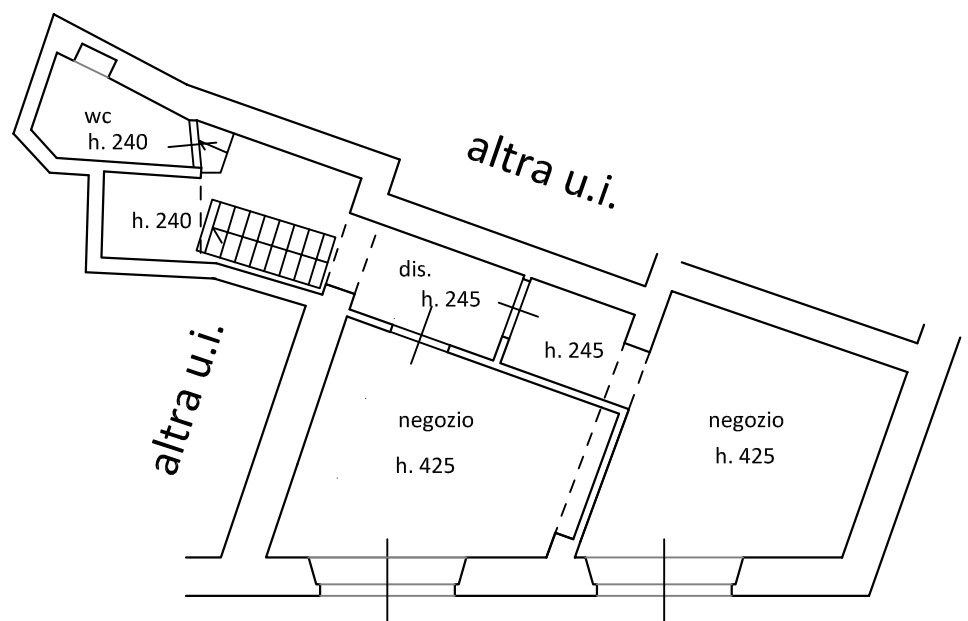
Piano terra
