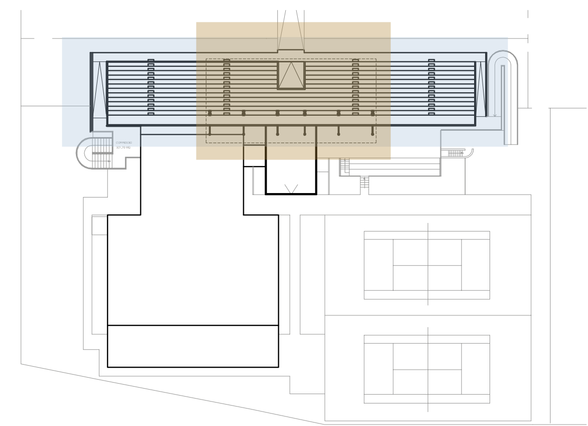
Pianta piano +6.00
